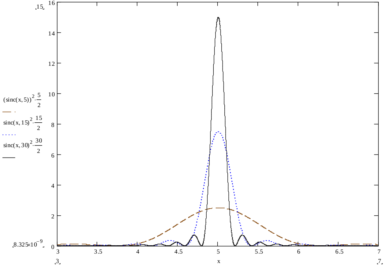
Figure 5.3. Plot of for various different values of t .
