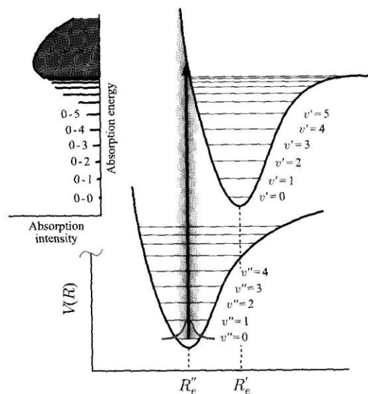
Figure 11.10. Potential energy surfaces leading to dissociation.
