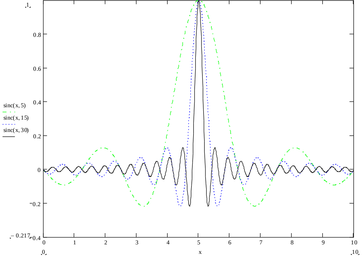
Figure 5.2. Plot of \text{sinc}\left(\left(\omega - \omega_{\bar{f}_i}\right)/2\right) for \omega_{\bar{f}_i} = 5 and different values of t .
