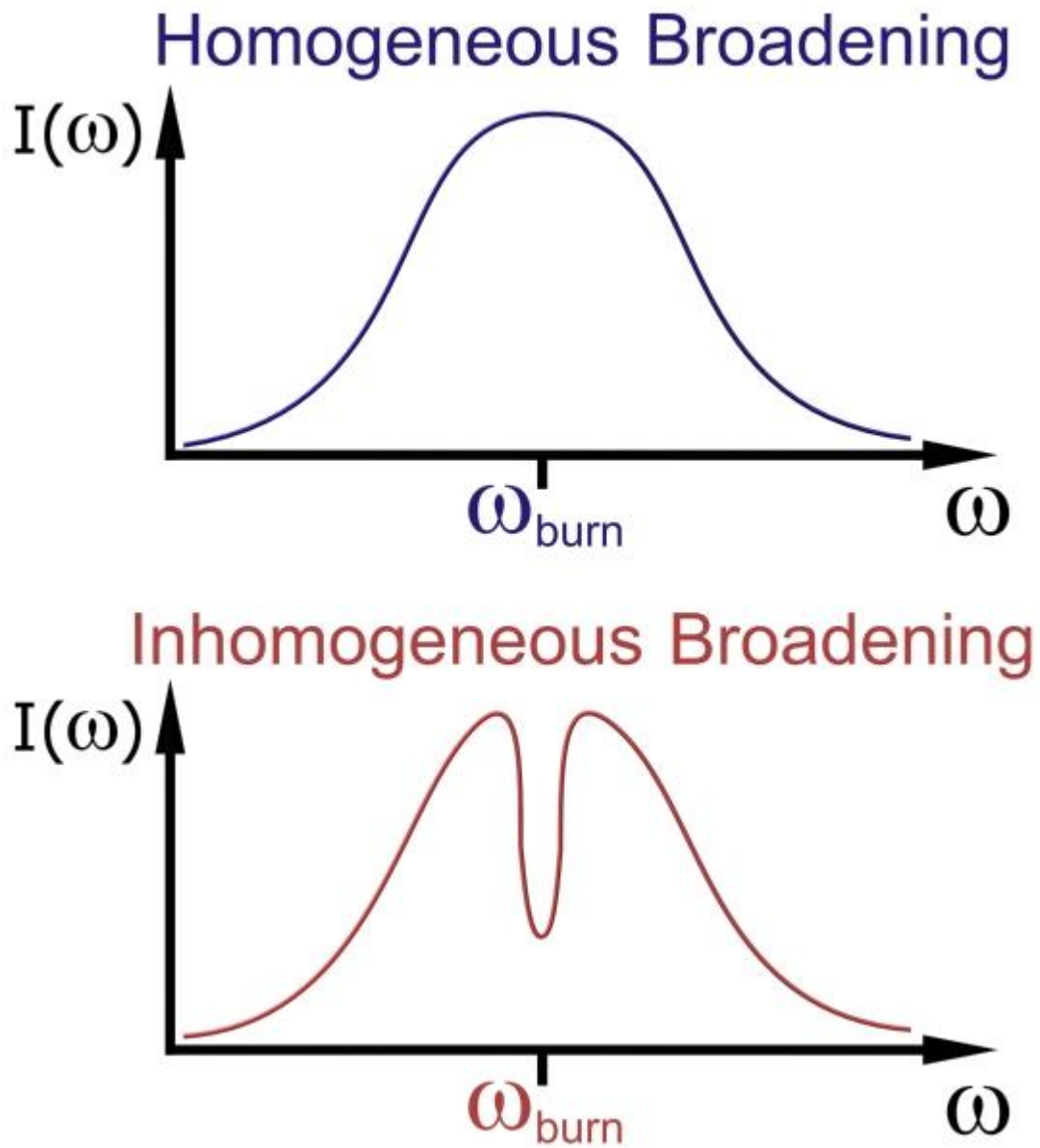
Figure 5.17. Hole burning for a system without significant inhomogeneous broadening and for a system in which inhomogeneous broadening is significant.
