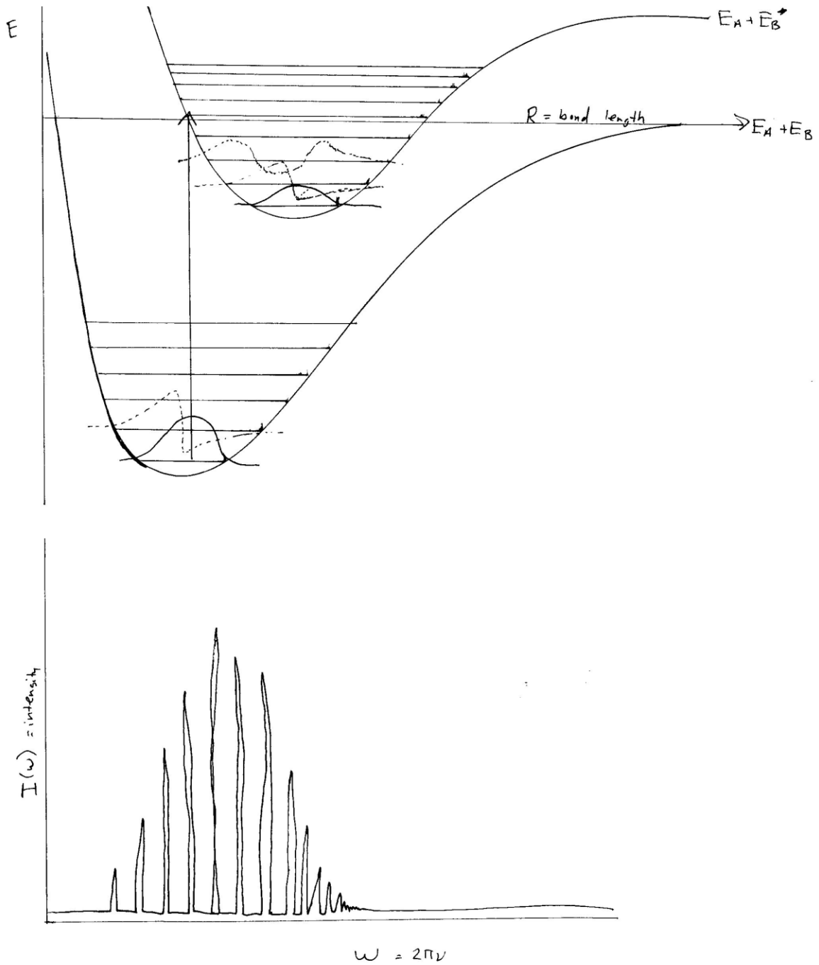
Figure 5.7: Schematic of the process of electronic excitation for a diatomic molecule. The curves denote the potential energy surfaces in the Born-Oppenheimer approximation, and the lines denote vibrational energy levels. A vibrationally resolved “spectrum” is sketched below the curve.
